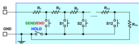
Figure 37. Remote Control Architecture
