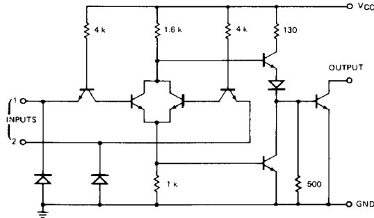
EQUIVALENT CIRCUIT (Each Driver)
