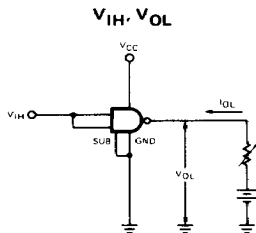
Both inputs are tested simultaneously. Fig. 1
