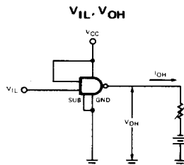
Each input is tested separately. Fig. 2
