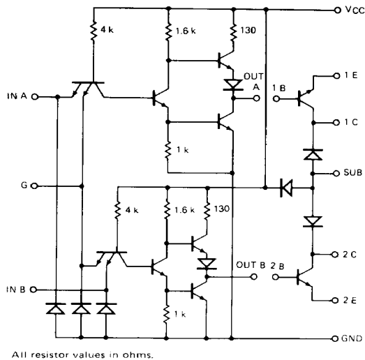
EQUIVALENT CIRCUIT
