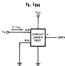
Each input is tested separately. Fig. 9
