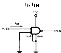
Each input is tested separately. Fig. 4
