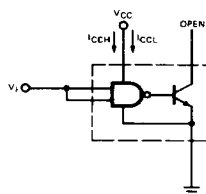
Both gates are tested simultaneously. Fig. 10
