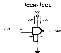
Both gates are tested simultaneously. Fig. 6
