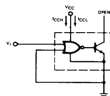
Both gates are tested simultaneously. Fig. 11
