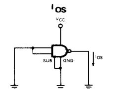
Each gate is tested separately. (55460/75460 only) Fig. 5
