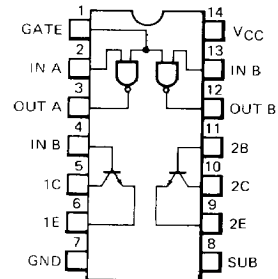
LOGIC FUNCTION
