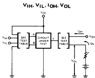
NOTE: Each input is tested separately.
