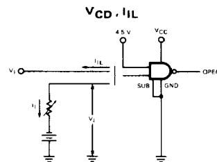
NOTES: A. Each input is tested separately. B. When testing V_{CD} , input not under test is open.
