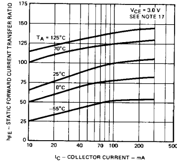
55460/75460 TRANSISTOR STATIC FORWARD CURRENT TRANSFER RATIO AS A FUNCTION OF COLLECTOR CURRENT
