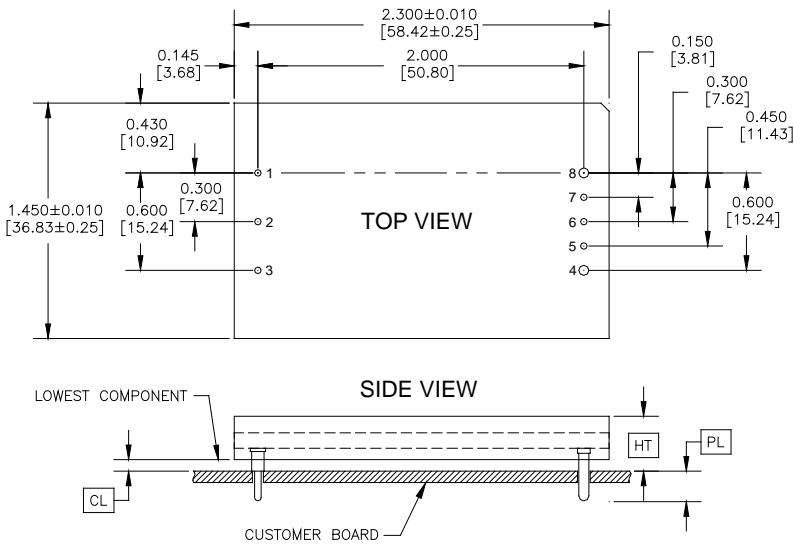
QM48T (Through-hole)
