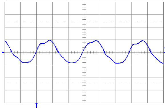
Fig. 12: Output voltage ripple (20 mV/div.) at full rated load current into a resistive load with C_o = 10\text{ }\mu\text{F} tantalum + 1 \mu\text{F} ceramic and V_{in} = 48\text{ V} . Time scale: 1 \mu\text{s} /div.
