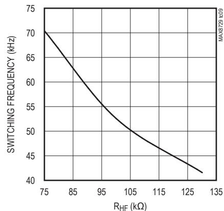
SWITCHING FREQUENCY vs. R_{HF}
