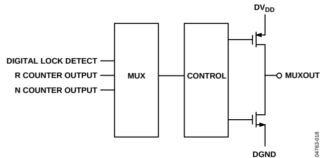
Figure 18. MUXOUT Circuit
