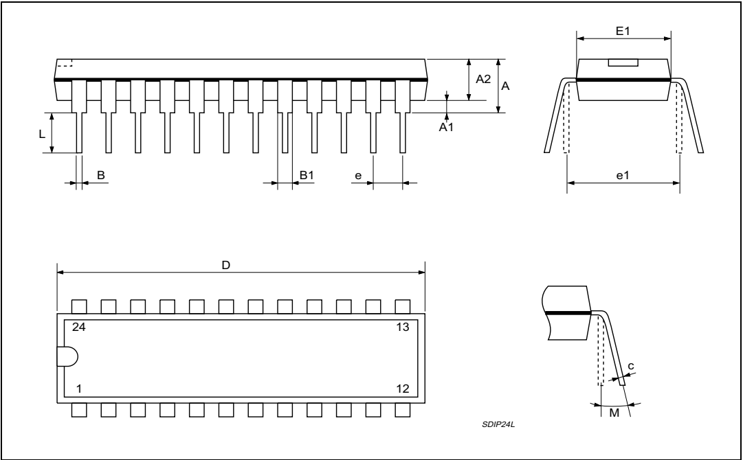
Figure 35. PowerDIP24 package outline
