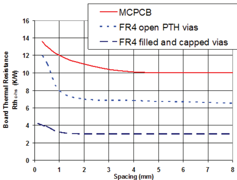
Figure 24. Comparison R_{\theta_{c-hs}} of various board technologies as a function of LED spacing.
