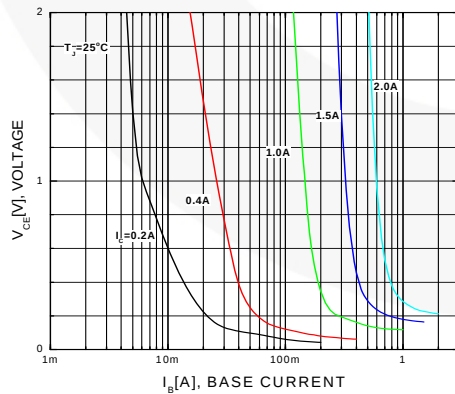
Figure 5. Typical Collector Saturation Voltage
