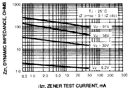
FIGURE 2 — TYPICAL ZENER IMPEDANCE
