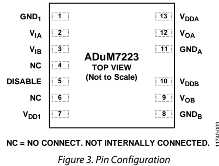
Figure 3. Pin Configuration
