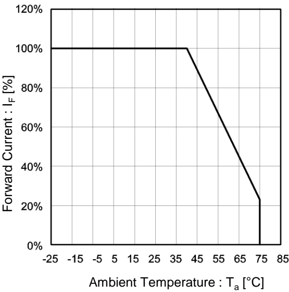
Fig.5 Derating
