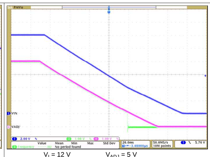
Figure 18. Power Down
