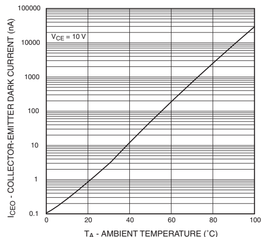
Fig. 4 Collector-Emitter Dark Current vs. Ambient Temperature
