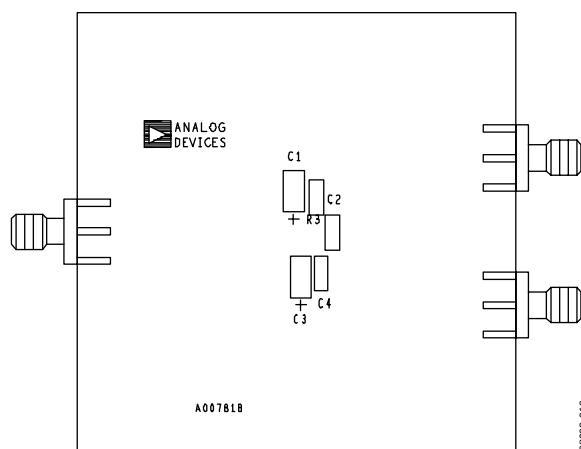
Figure 12. Assembly Drawing, Circuit Side
