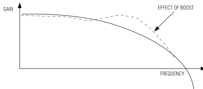
Figure 2b. Cable Booster Using the MAX4023/MAX4025
