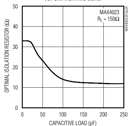
OPTIMAL ISOLATION RESISTOR vs. CAPACITIVE LOAD
