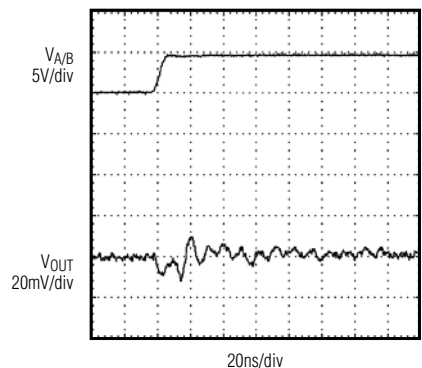
CHANNEL SWITCHING TRANSIENT
