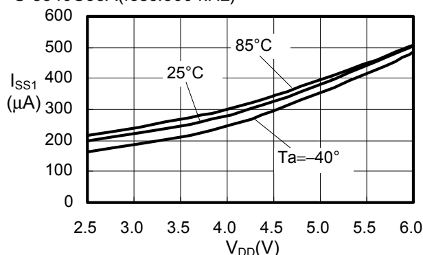
S-8340C33A(fosc:300 kHz)
