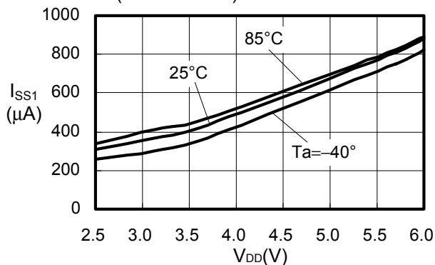
S-8340A33A(fosc:600 kHz)
