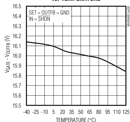
GATE TO OUTFB CLAMP VOLTAGE vs. TEMPERATURE
