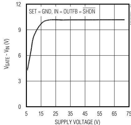
GATE VOLTAGE vs. SUPPLY VOLTAGE
