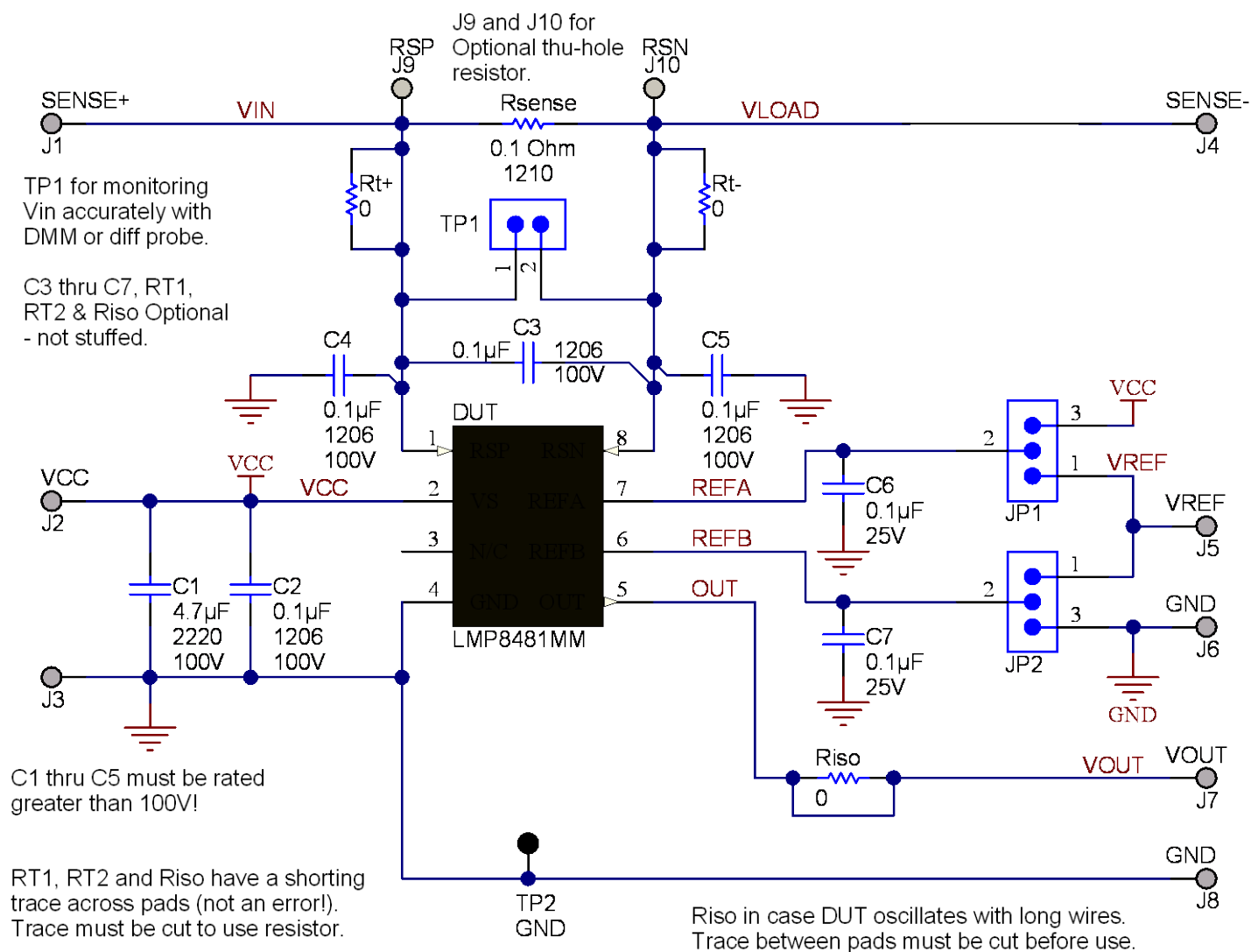
Figure 10: EVM Schematic
