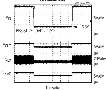
UNDERVOLTAGE PULSE (5V/2.2MHz)
