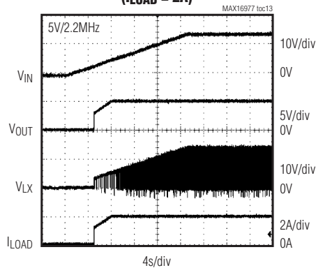
OUTPUT RESPONSE TO SLOW INPUT RAMP ( I_{LOAD} = 2A )
