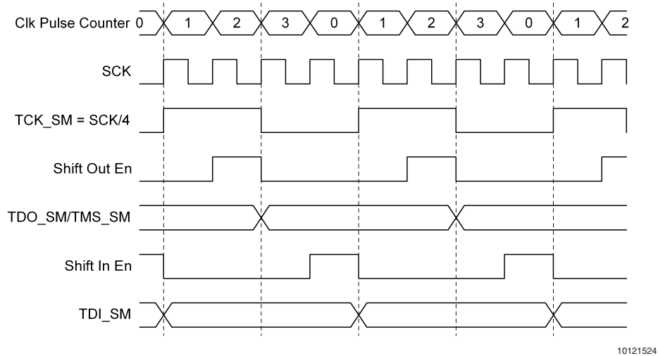
FIGURE 5. Shift Register Implementation and Timing
