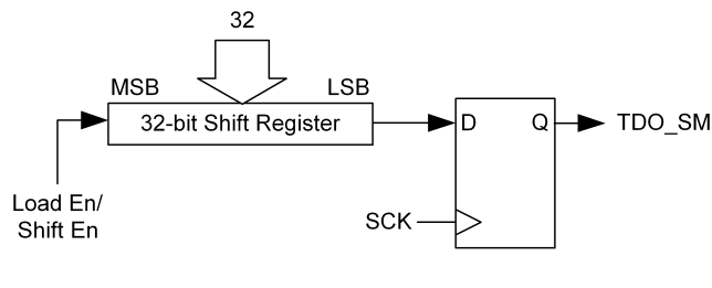
FIGURE 3. TDO_SM Shifter
