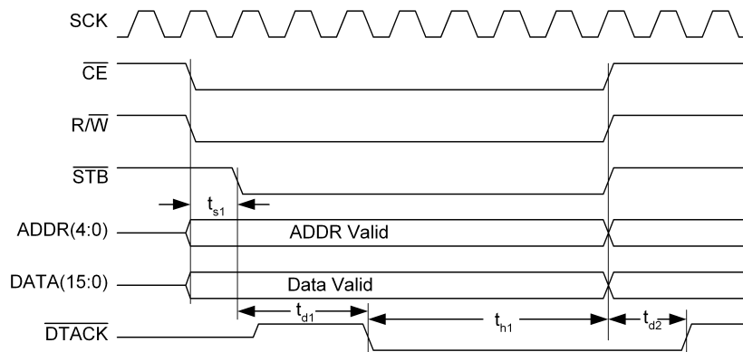
FIGURE 11. PPI Write Cycle Timing Diagram
