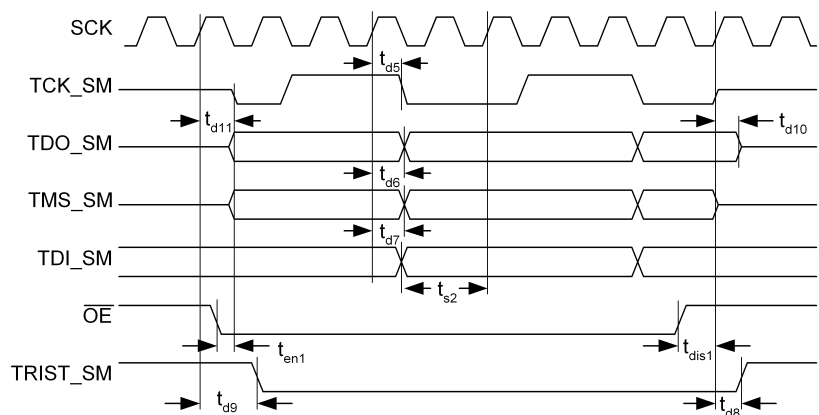
FIGURE 13. SSI Timing Diagram with Clock Divider set to 4
