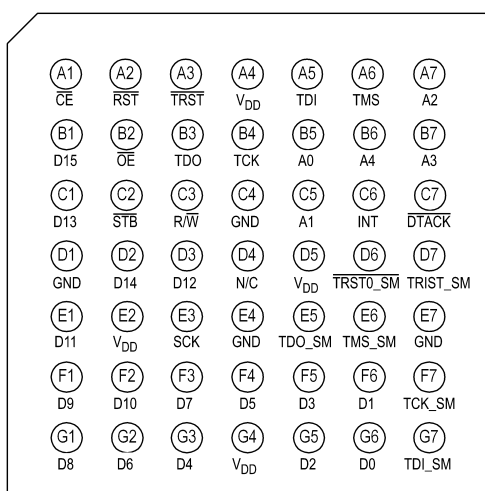
BGA Package Pinout (Top View)
