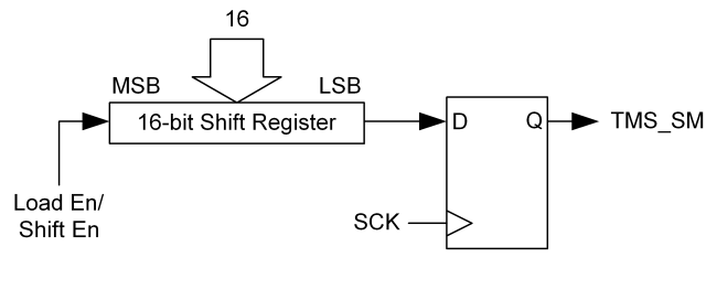
FIGURE 2. TMS_SM Shifter
