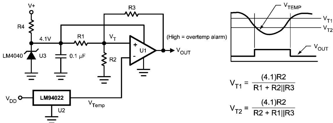
FIGURE 4. Celsius Thermostat
