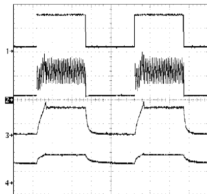
\overline{\text{SHDN}} Pin Duty Cycle Control Waveforms
