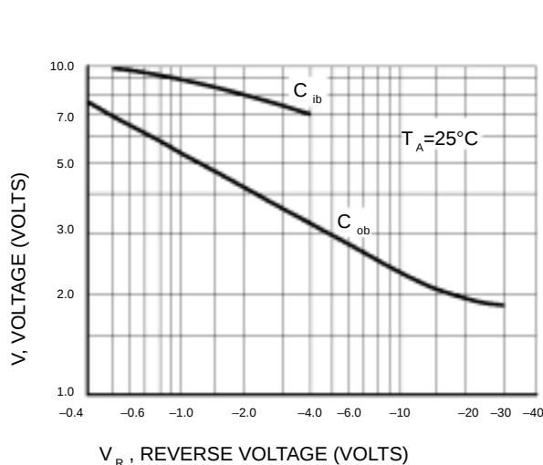
Figure 5. Capacitances
