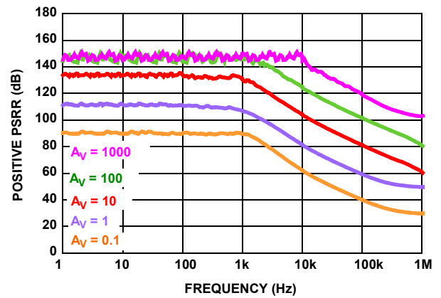
FIGURE 24. POSITIVE PSRR V_{E0} AND V_{C0} ( R_F = 30.1k )
