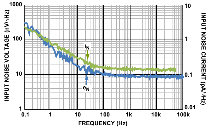
FIGURE 30. INPUT VOLTAGE AND CURRENT NOISE
