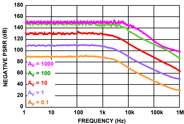
FIGURE 25. NEGATIVE PSRR V_{E0} AND V_{C0} ( R_F = 30.1k )
