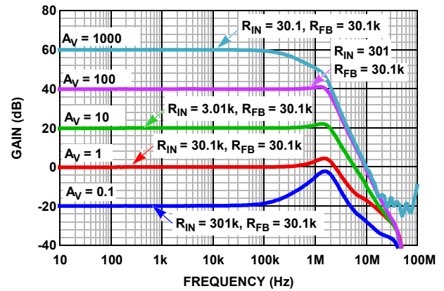
FIGURE 18. CLOSED LOOP GAIN ( R_{FB} = 30.1k ) vs FREQUENCY
