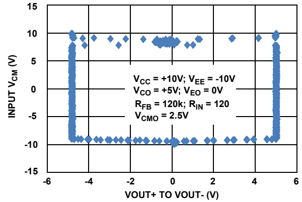
FIGURE 16. COMMON MODE RANGE vs OUTPUT VOLTAGE
