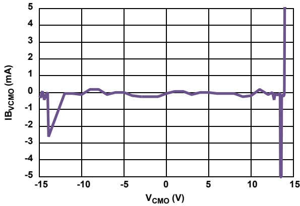
FIGURE 15. IB_{V_{CMO}} vs V_{CMO} INPUT VOLTAGE RANGE
