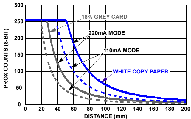
FIGURE 8. PROX COUNTS vs DISTANCE WITH 10CM x 10CM REFLECTOR
