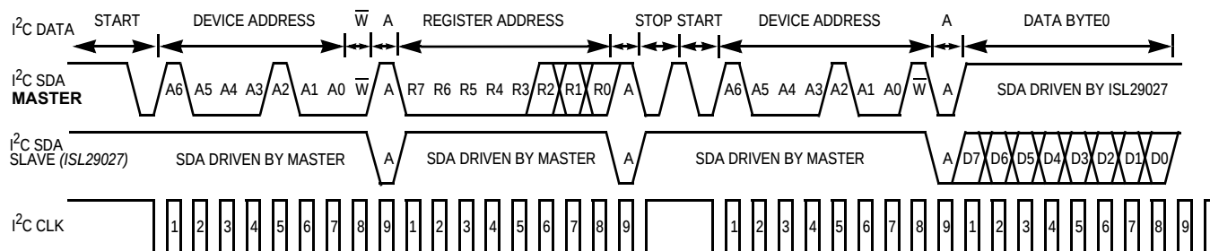
FIGURE 3. I²C DRIVER TIMING DIAGRAM FOR MASTER AND SLAVE CONNECTED TO COMMON BUS
