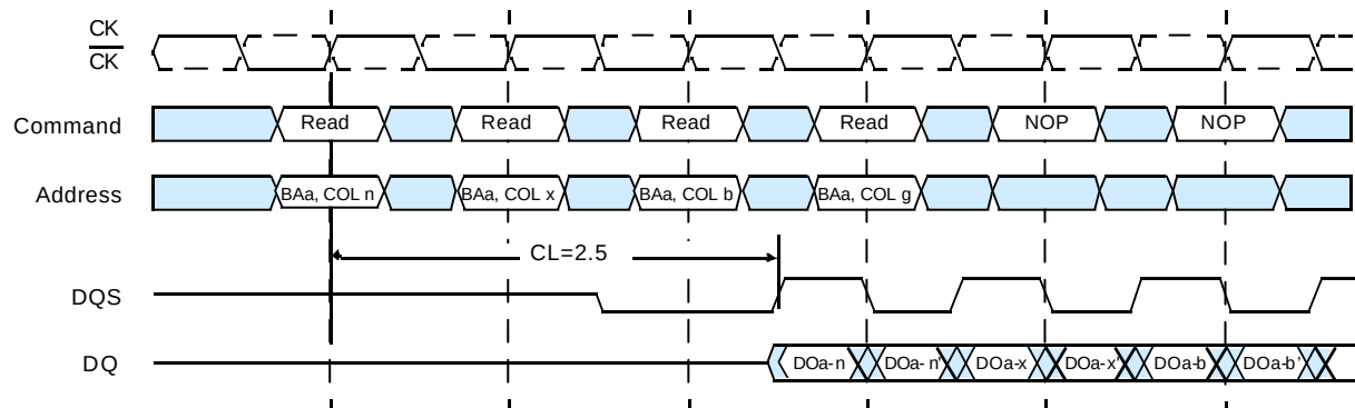
CAS Latency = 2.5
