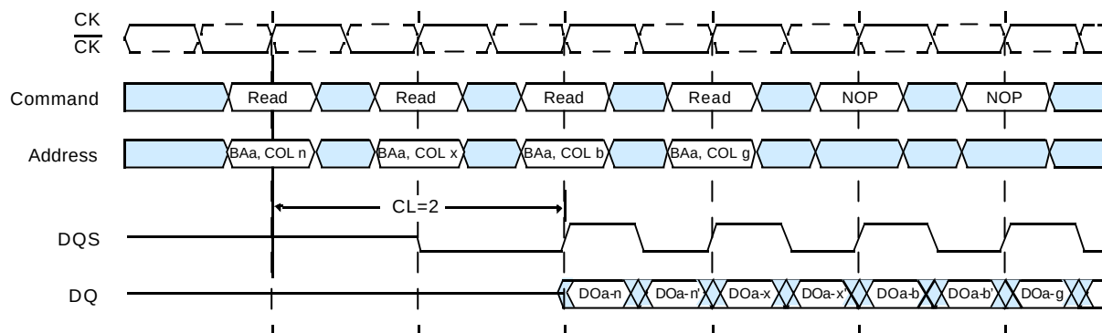
CAS Latency = 2
