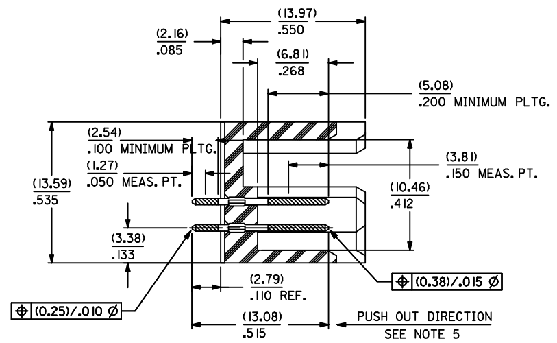
SECTION W-W
