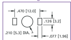
Mounting Detail
