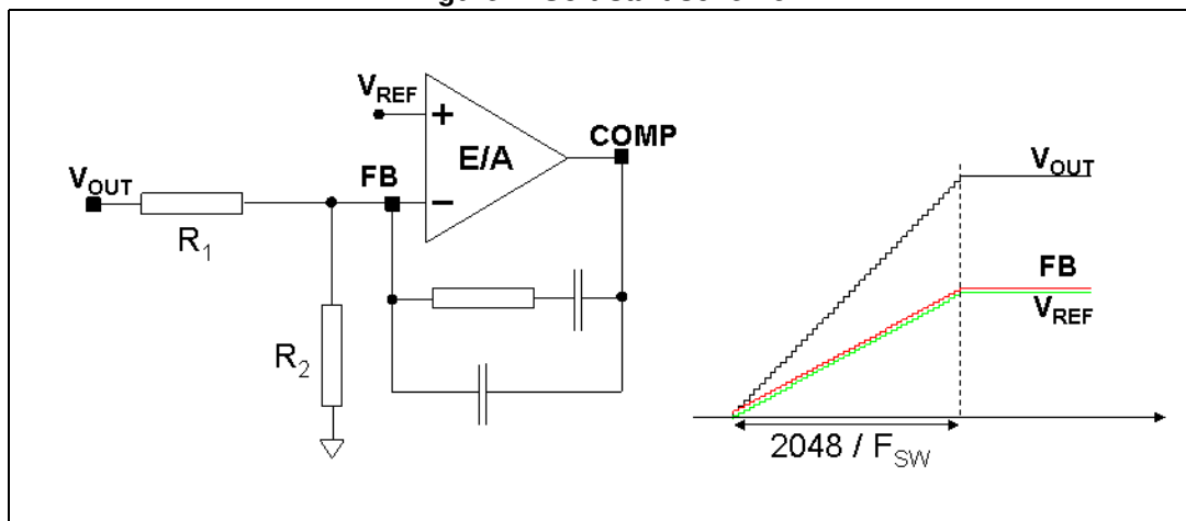
Figure 7. Soft-start scheme
