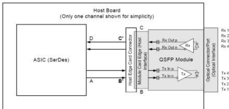
Figure 19. Connection between Mellanox® ConnectX-3* and QSFP
