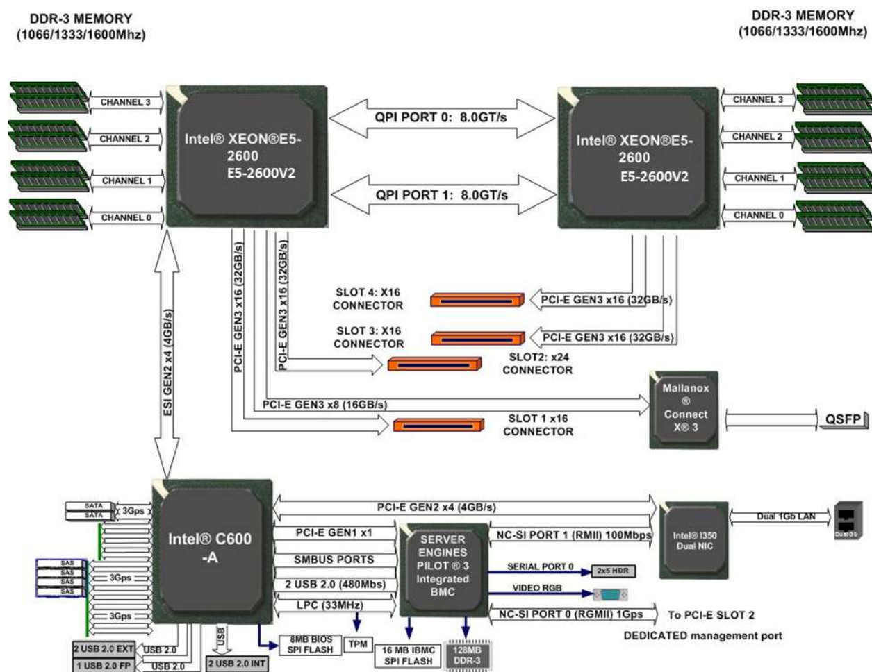
Figure 5. Intel® Server Board S2600WPQ/S2600WPF Functional Block Diagram
