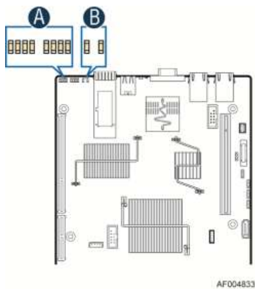
Figure 57. Rear Panel Diagnostic LEDs (Block A)
