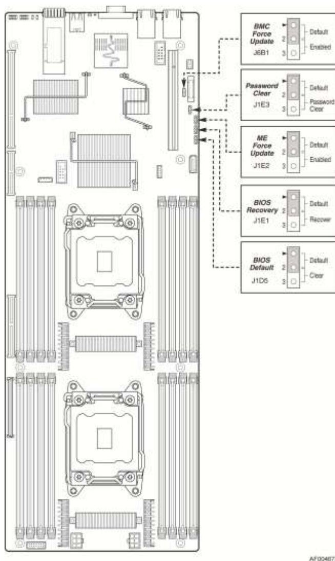
Figure 54. Jumper Blocks (J6B1, J1E2, J1E3, J1E1, J1D5)
