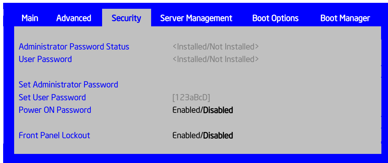
Figure 41. Security Screen
