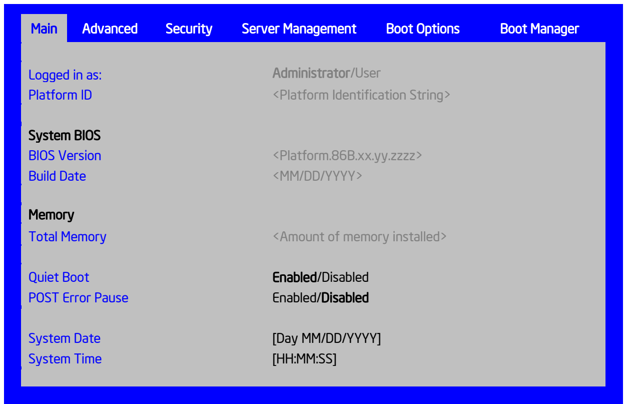
Figure 23. Main Screen
