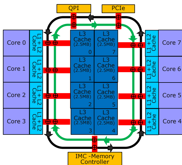
Figure 9. Processor with IMC Functional Block Diagram
