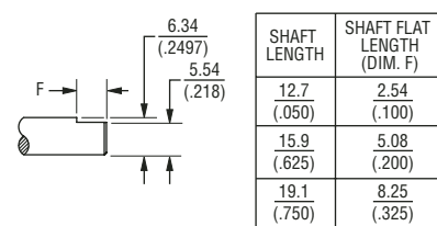
Shaft End Style C
