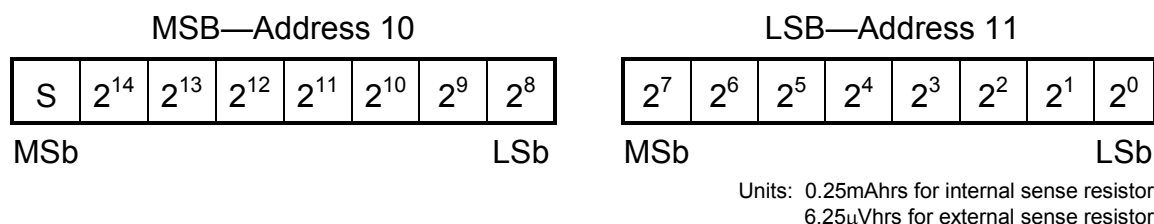
Figure 4. CURRENT ACCUMULATOR FORMAT
