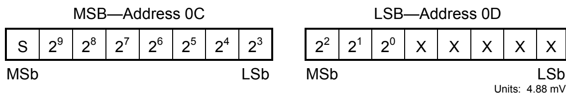
Figure 6. VOLTAGE REGISTER FORMAT
