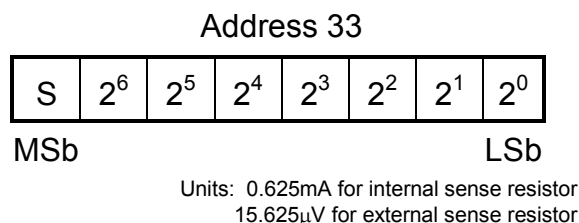
Figure 5. CURRENT OFFSET BIAS
