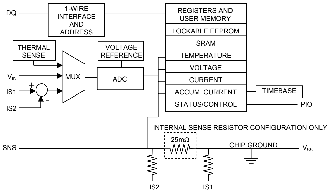
Figure 1. FUNCTIONAL DIAGRAM
