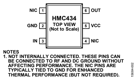
Figure 2. Pin Configuration
