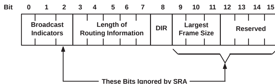
Figure 6. Routing-Control Field
