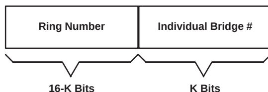
Figure 7. Route-Designator Field
