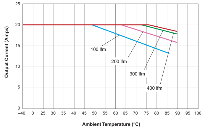
ULQ-2.5/20-D48
