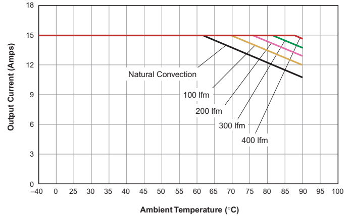
ULQ-2.5/15-D48
