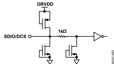
Figure 38. Equivalent SDIO/DCS Input Circuit
