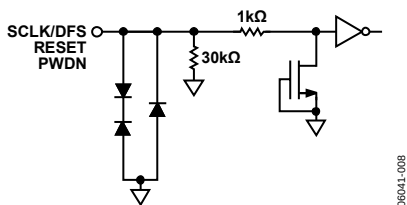
Figure 35. Equivalent SCLK/DFS, RESET, PWDN Input Circuit
