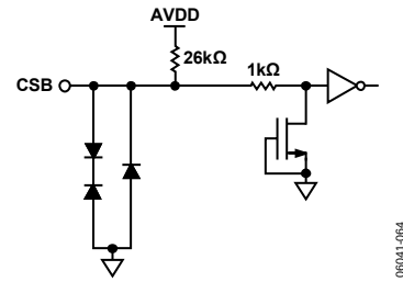
Figure 36. Equivalent CSB Input Circuit
