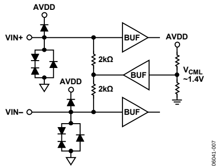
Figure 34. Analog Inputs ( V_{CM} \approx 1.4\text{ V} )
