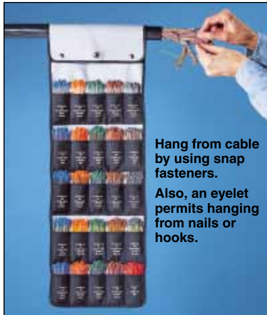
PANDUIT PAN-POUCH PPC25x50F filled with color-coded PAN-TY Cable Ties is shown.
