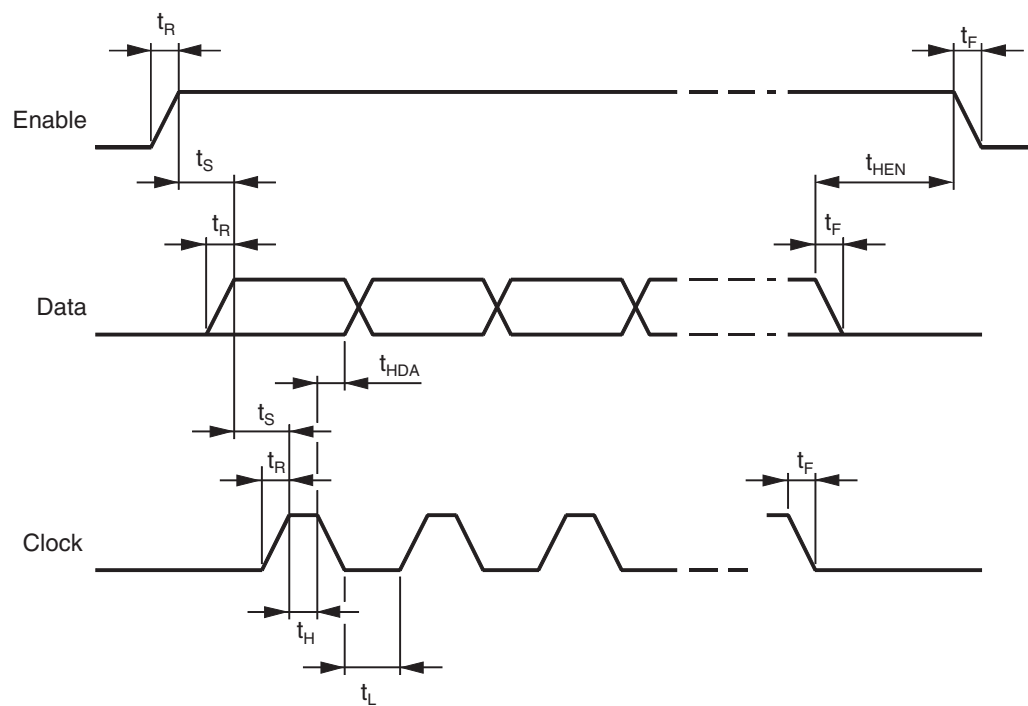
Figure 3-9. Bus Timing
