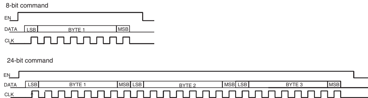
Figure 3-8. Pulse Diagram
