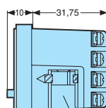
① Mounting
