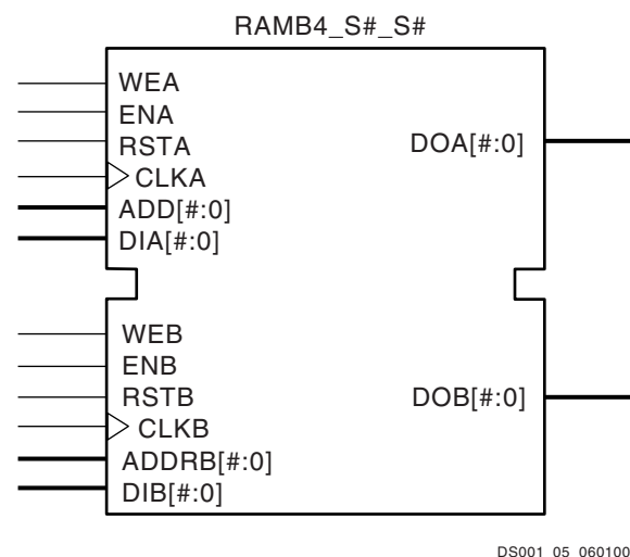
Figure 8: Dual-Port Block RAM
