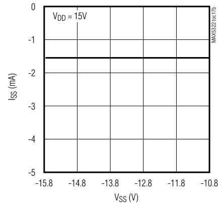
BIPOLAR NEGATIVE SUPPLY CURRENT vs. SUPPLY VOLTAGE
