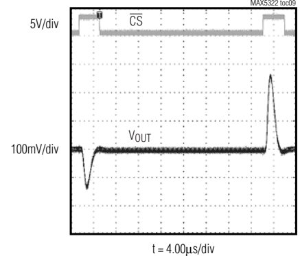
BIPOLAR MAJOR CARRY GLITCH ENERGY, C_{LOAD} = 250\text{pF}
