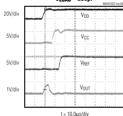
UNIPOLAR STARTUP RESPONSE, C_{LOAD} = 230pF
