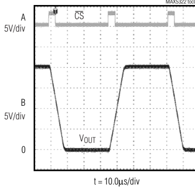
BIPOLAR SETTLING TIME ( C_{LOAD} = 250\text{pF} , R_{LOAD} = 2\text{k}\Omega )
