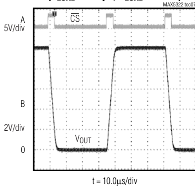
UNIPOLAR SETTLING TIME ( C_{LOAD} = 250\text{pF} , R_{LOAD} = 10\text{k}\Omega )
