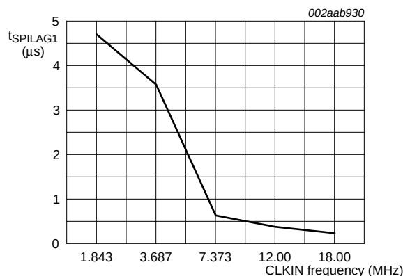
Fig 23. t_{\text{SPILAG1}} as a function of CLKIN frequency
