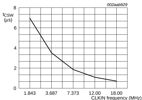
Fig 22. t_{\text{CSW}} as a function of CLKIN frequency
