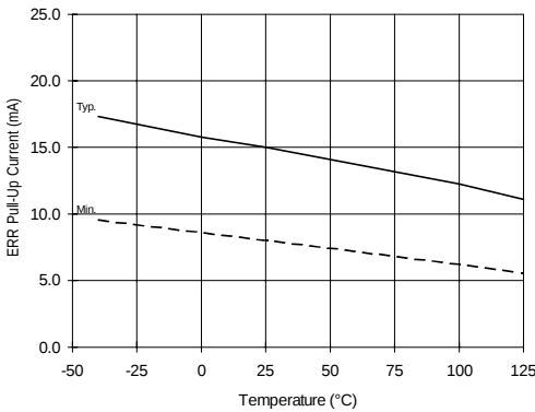
Figure 32A. ERR Pull-Up Current vs. Temperature
