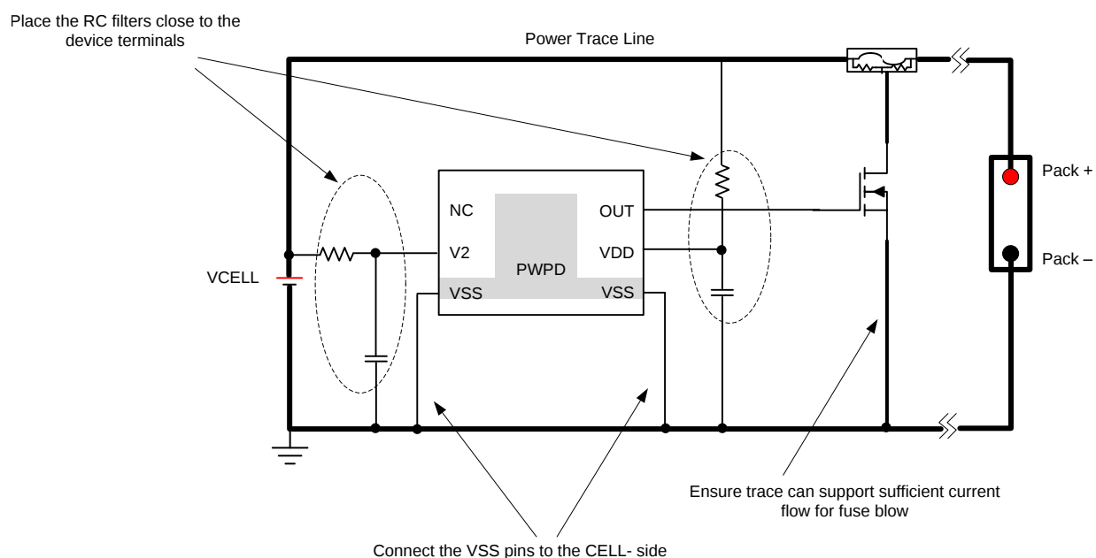
Figure 14. Layout Schematic
