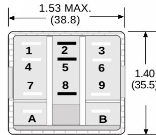
OUTLINE DIMENSIONS DIMENSIONS SHOWN IN INCHES & (MILLIMETERS).
