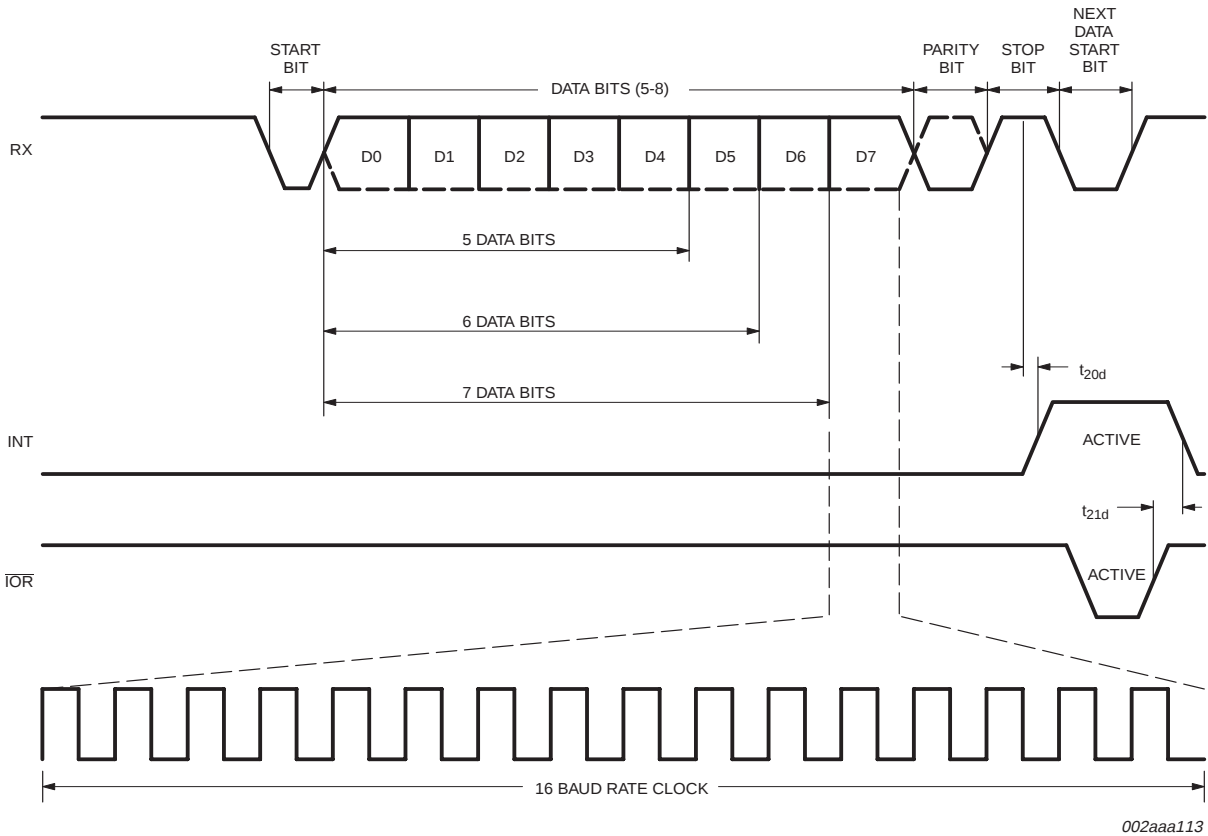
Fig 11. Receive timing.
