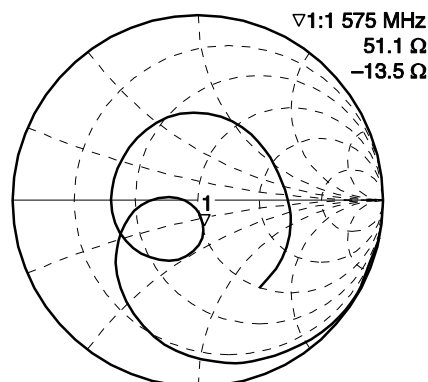
S 22 —FREQUENCY
