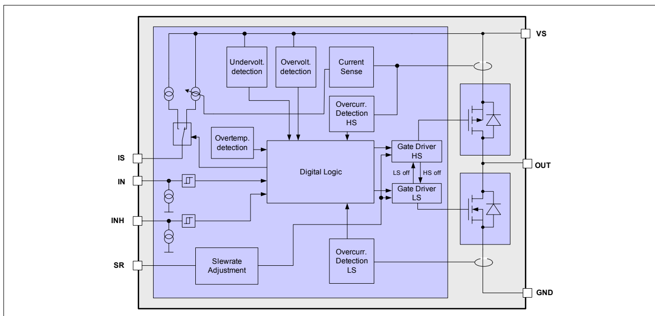
Figure 1 Block Diagram
