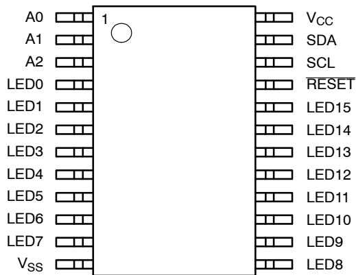
SOIC (W), TSSOP (Y) (Top View)
