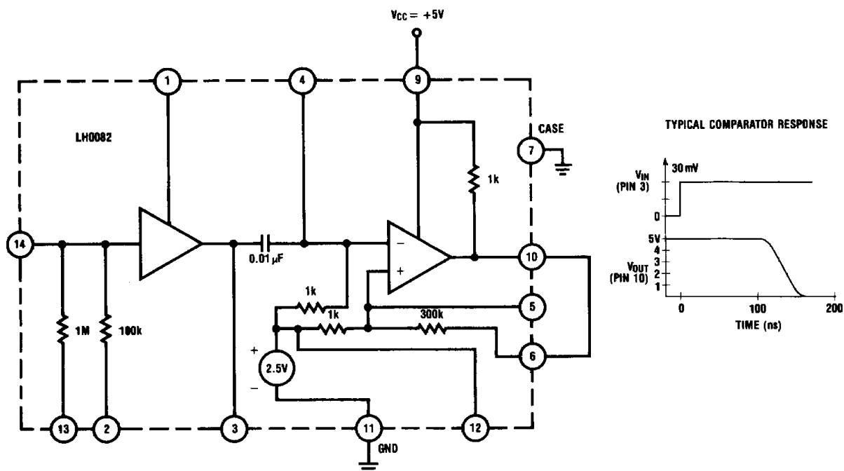
FIGURE 2. Comparator Test Circuit
