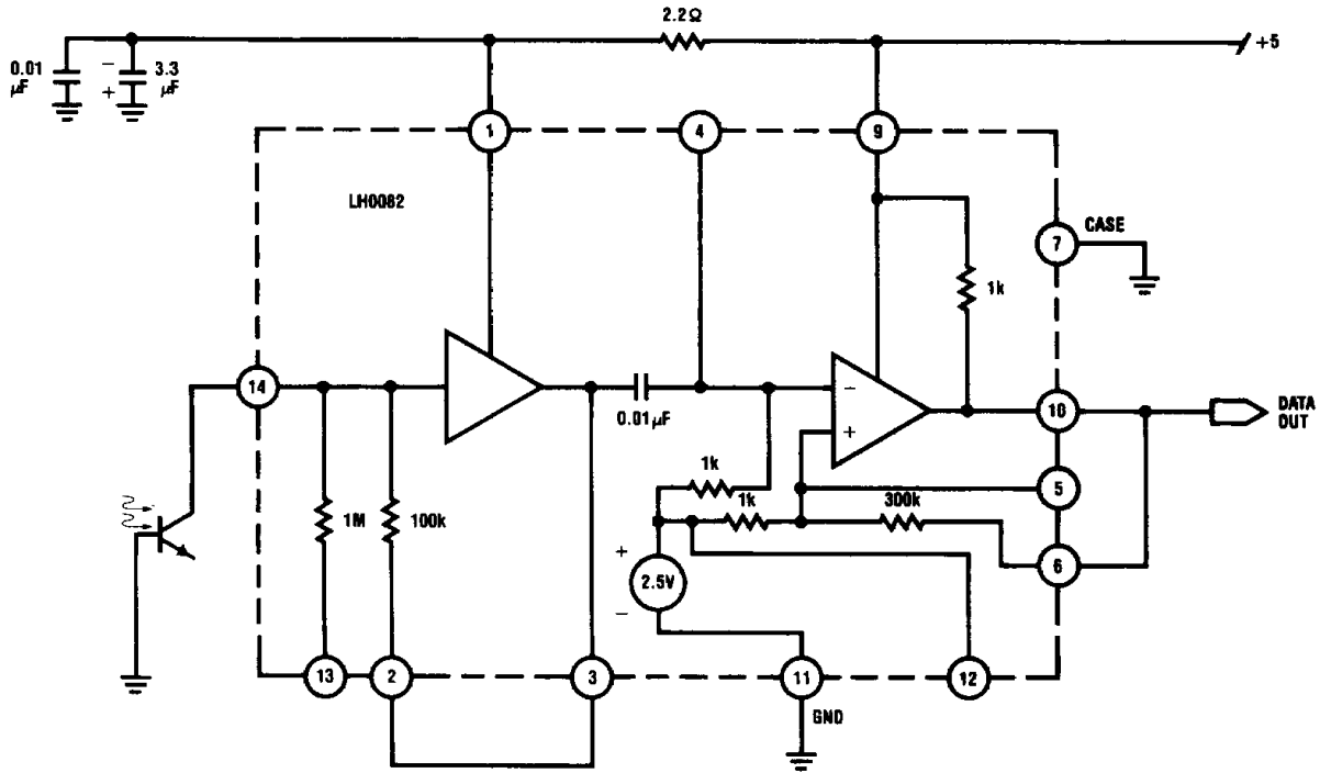
FIGURE 8. Connection to Phototransistor—Low Sensitivity, High Speed Receiver
