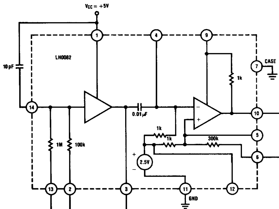
FIGURE 1. Preamp Test Circuit
