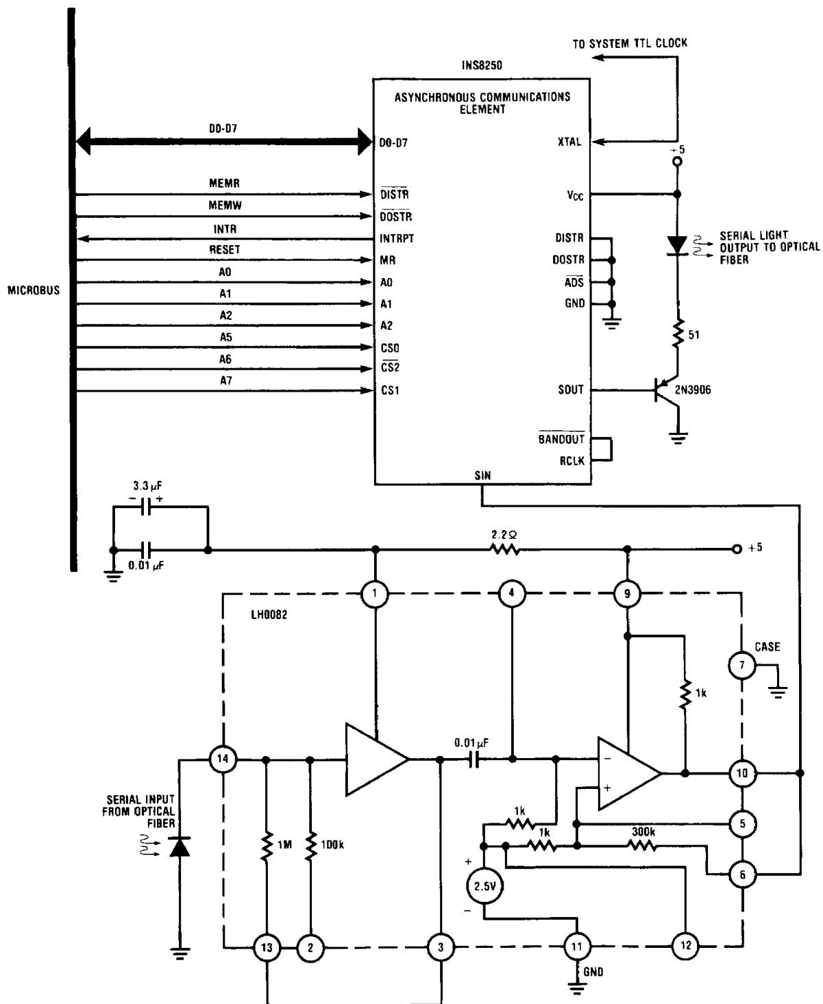
FIGURE 10. Optical Link to Microbus
