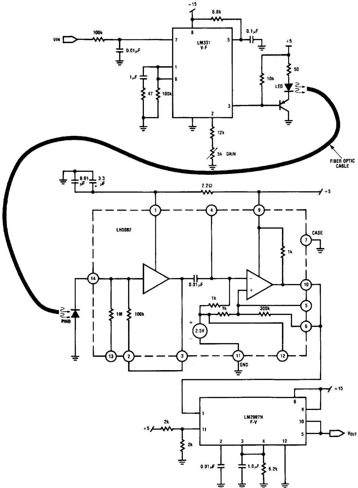
FIGURE 11. Analog Data Link Using V/F and F/V
