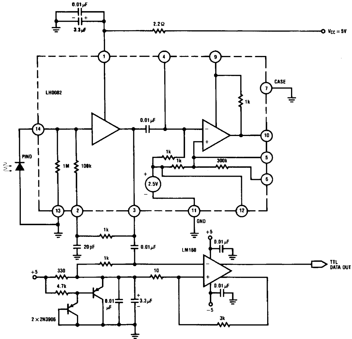
FIGURE 5. High Speed—Low Sensitivity Receiver
