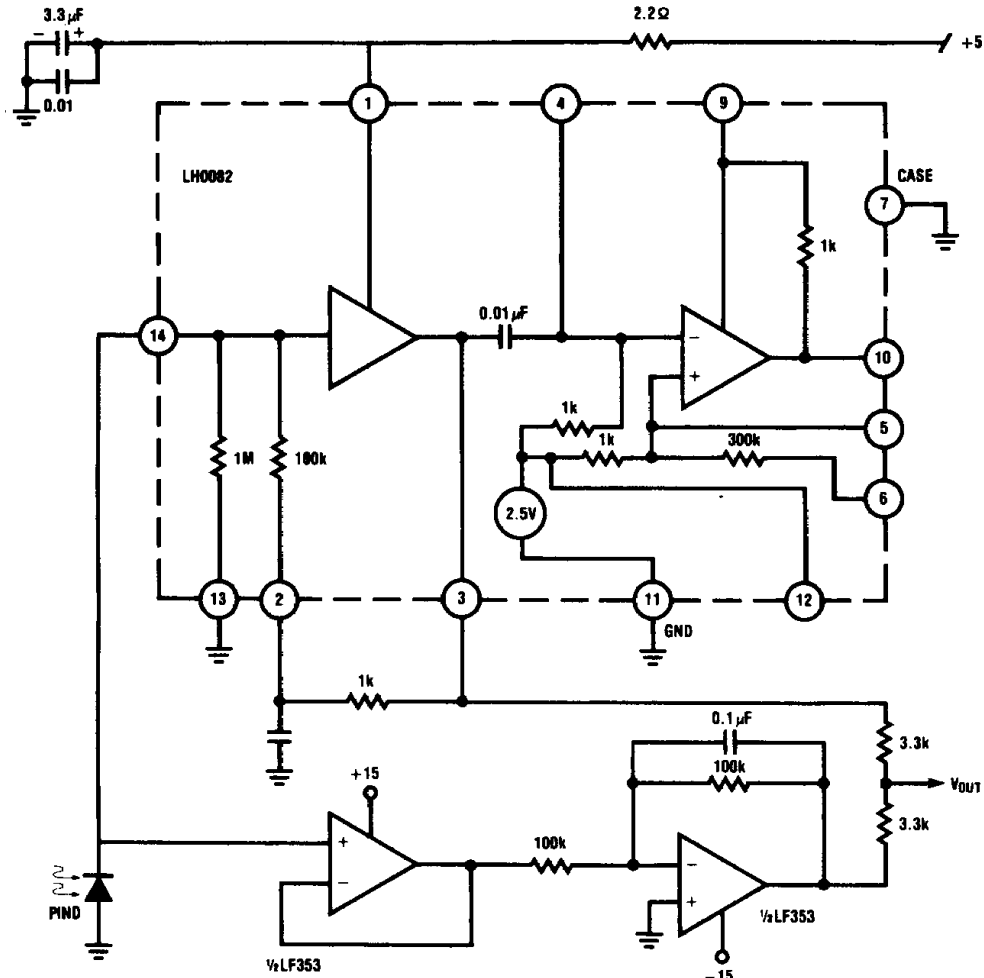
FIGURE 12. Low Temperature Drift Analog Receiver
