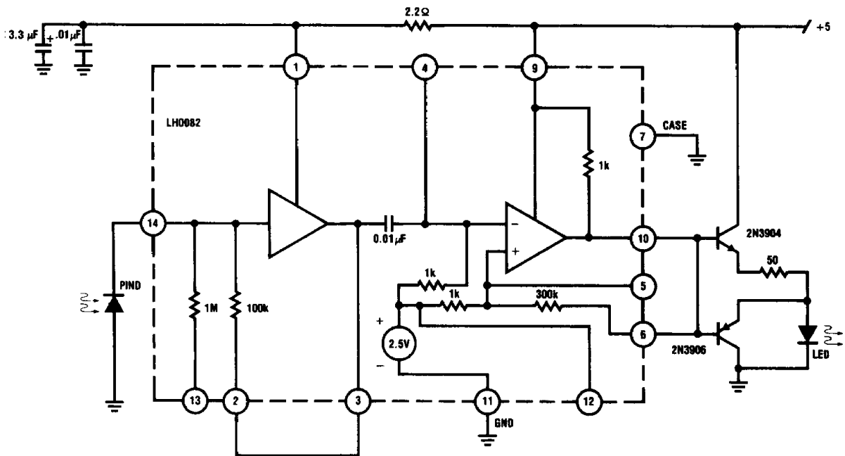
FIGURE 9. Fiber-Optic Link Repeater
